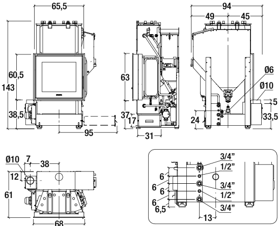
Model: MP973 TH ACS
