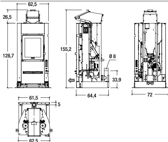
Model: MP980 WF
