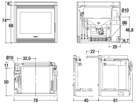
Model: IP 14 TH G
