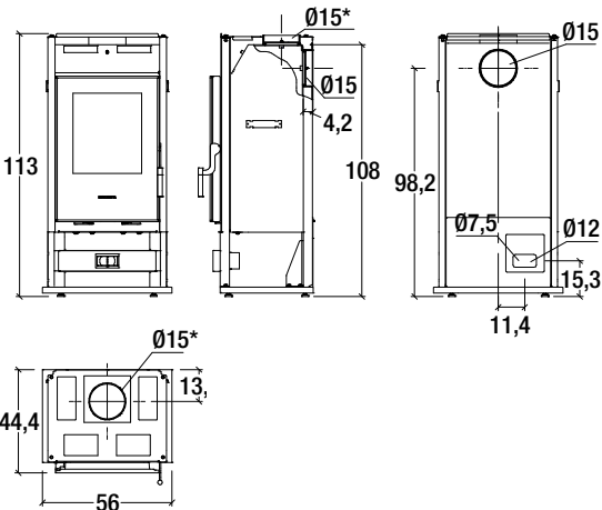
Model: E928 WF
