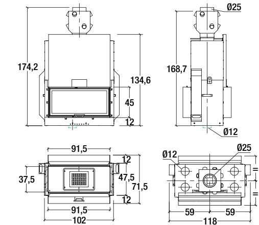
Model: ME 90 B
