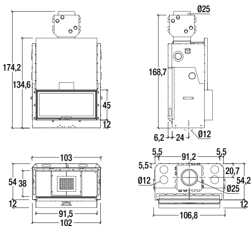
Model: ME 90 Con mantello cappa / With hood cover
