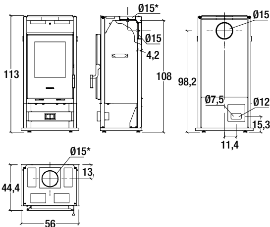
Model: E928 WF BCS
