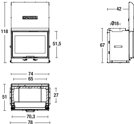
Model: MC 70/51 SL
