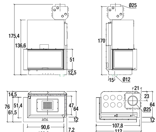
Model: ME 90 D, ME 90 S
