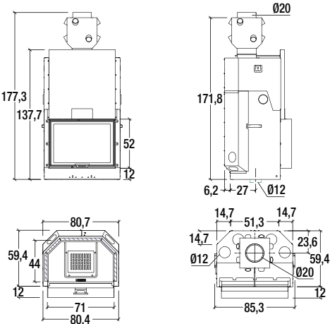
Model: ME 70 Con mantello cappa / With hood cover
