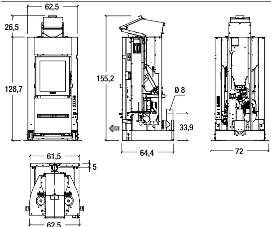
Model: MP980-S WF
