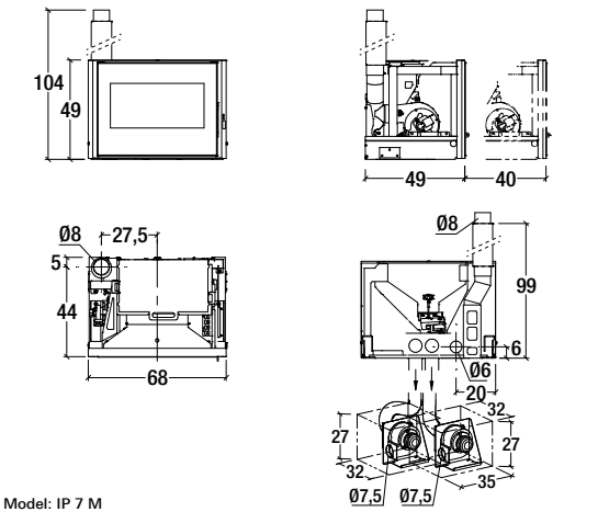
Model: IP 7 M
