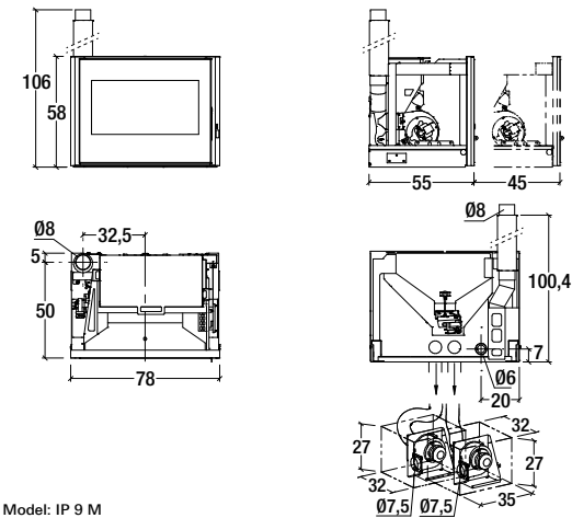
Model: IP 9 M
