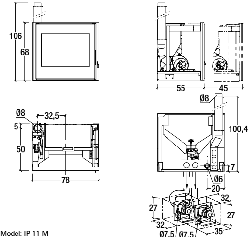
Model: IP 11 M
