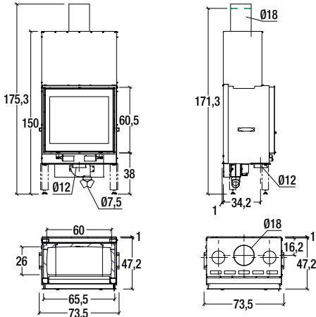
Model: MC 65/60 PLUS Con mantello cappa / With hood cover
