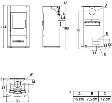
Model: E928 ST
