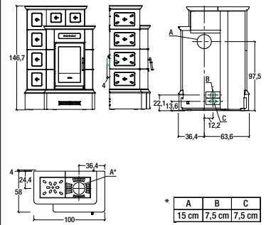
Model: ORTISEI BCS
