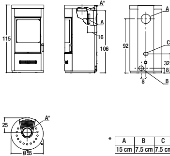
Model: E929 M Hermetic
