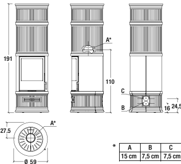
Model: E929 C-H Hermetic
