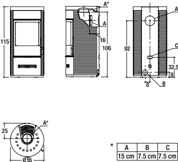
Model: E929 D BCS
