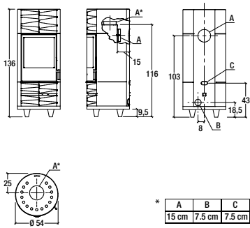
Model: ROUND-M Hermetic
