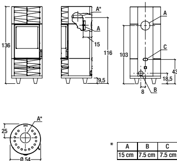
Model: ROUND-M BCS
