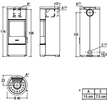
Model: E924 BCS
