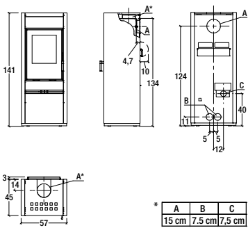
Model: E928 A BCS
