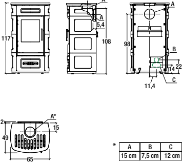
Model: E928 R
