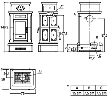
Model: CANAZEI BCS
