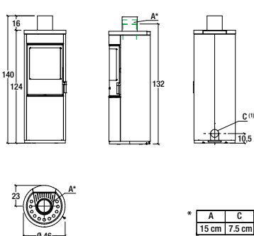
Model: E924 A Hermetic
