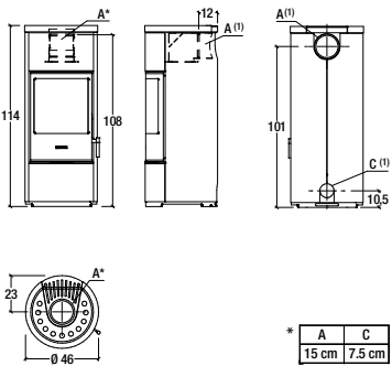
Model: E924 Hermetic
