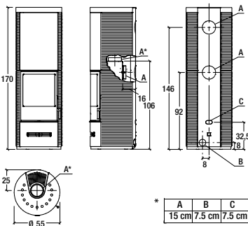
Model: E929 D-H BCS
